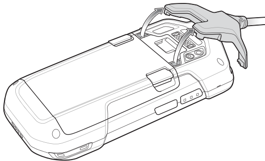
Figure 142: Remove Cable from TC70
