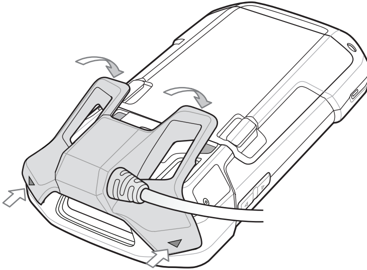
Figure 124: Audio Adapter Installation
