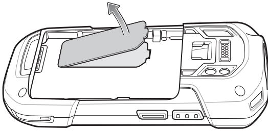
Figure 16: Remove Access Door
