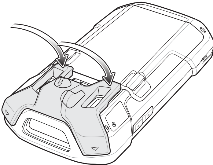
Figure 119: Rotate Audio Adapter onto TC70
