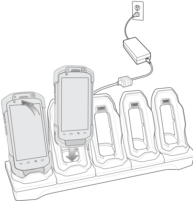
Figure 110: TC70 Battery Charging
