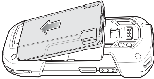
Figure 10: Insert Bottom of Battery into Battery Compartment
