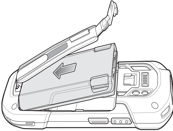
Figure 7: Insert Bottom of Battery into Battery Compartment
