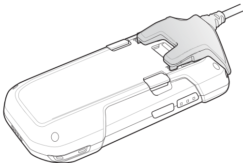
Figure 130: Cable Attached to TC70
