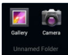
Figure 31: Open Folder
